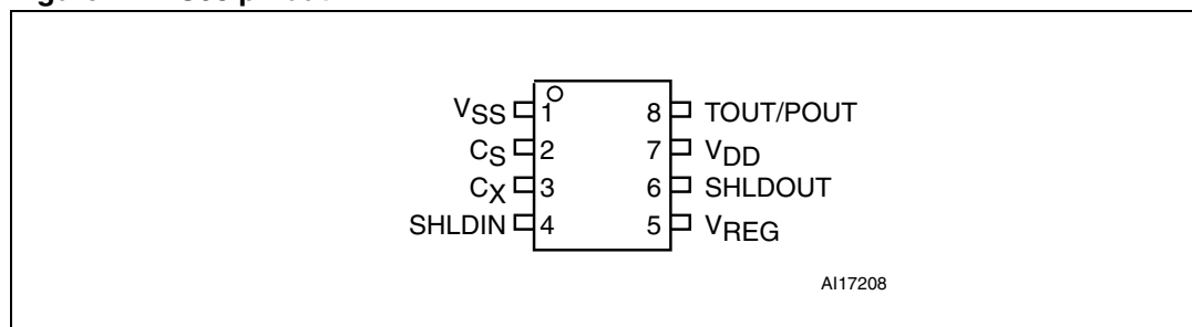
Figure 2. S08 pinout
