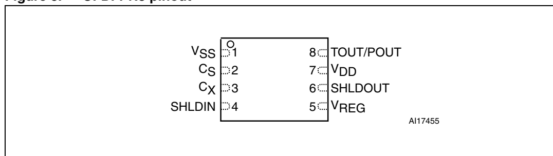
Figure 3. UFDFPN8 pinout
